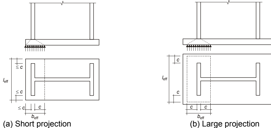
Figure 6.4: Area of equivalent T-Stub in compression
