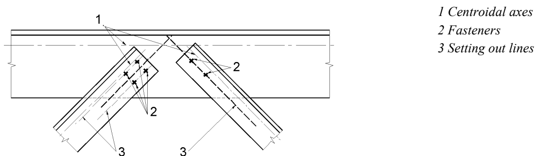
Figure 2.1: Setting out lines
