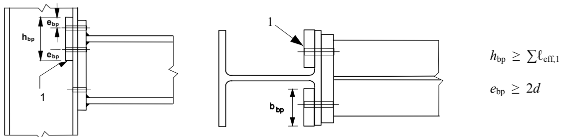
1 Backing plate
