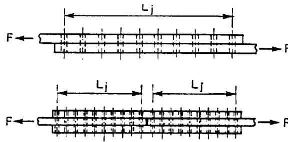
Figure 3.7: Long joints
