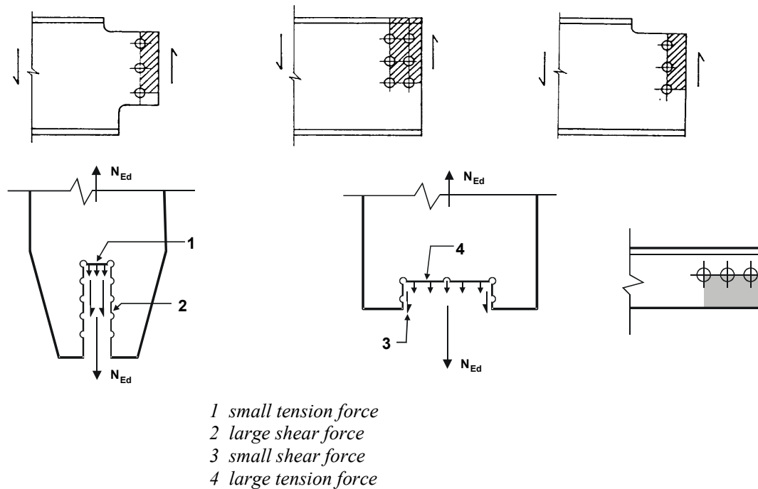
Figure 3.8: Block tearing
